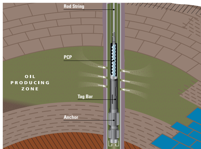
Typical PC Pump Installation
