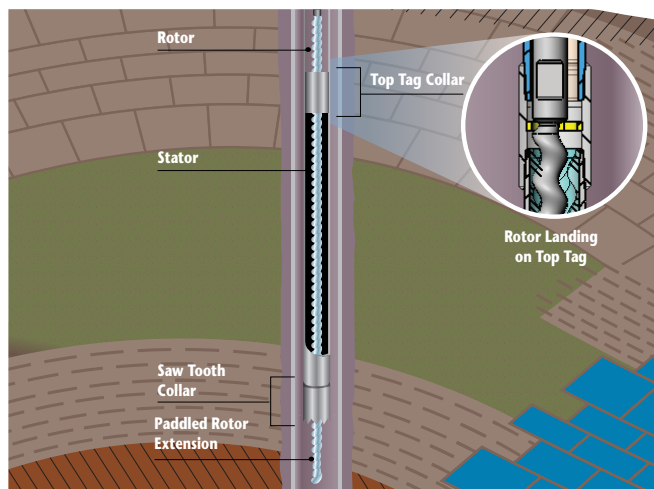
Top Tag Installation
